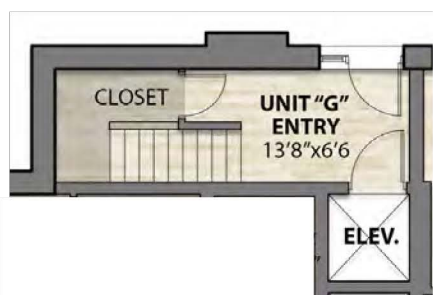
First Floor Plan - Unit Entry
